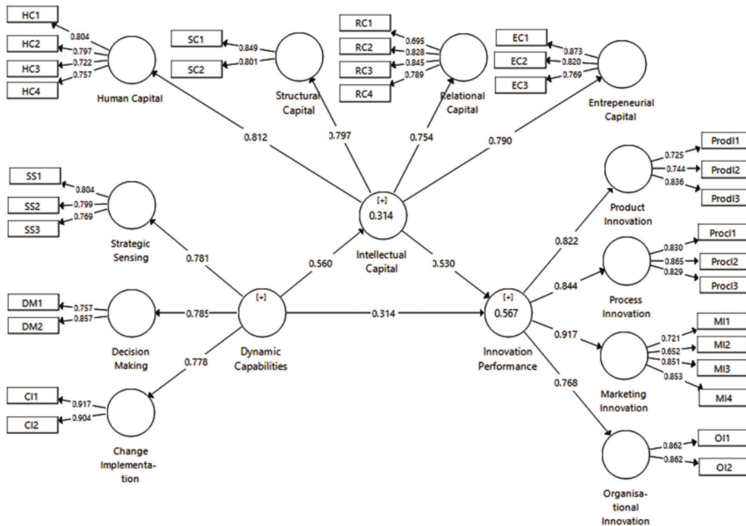
Figure 2. Path model
