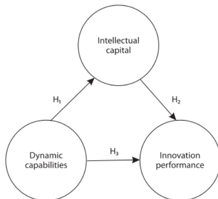
Figure 1. Research model
